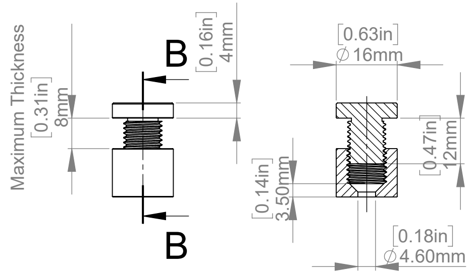
SECTION B-B
