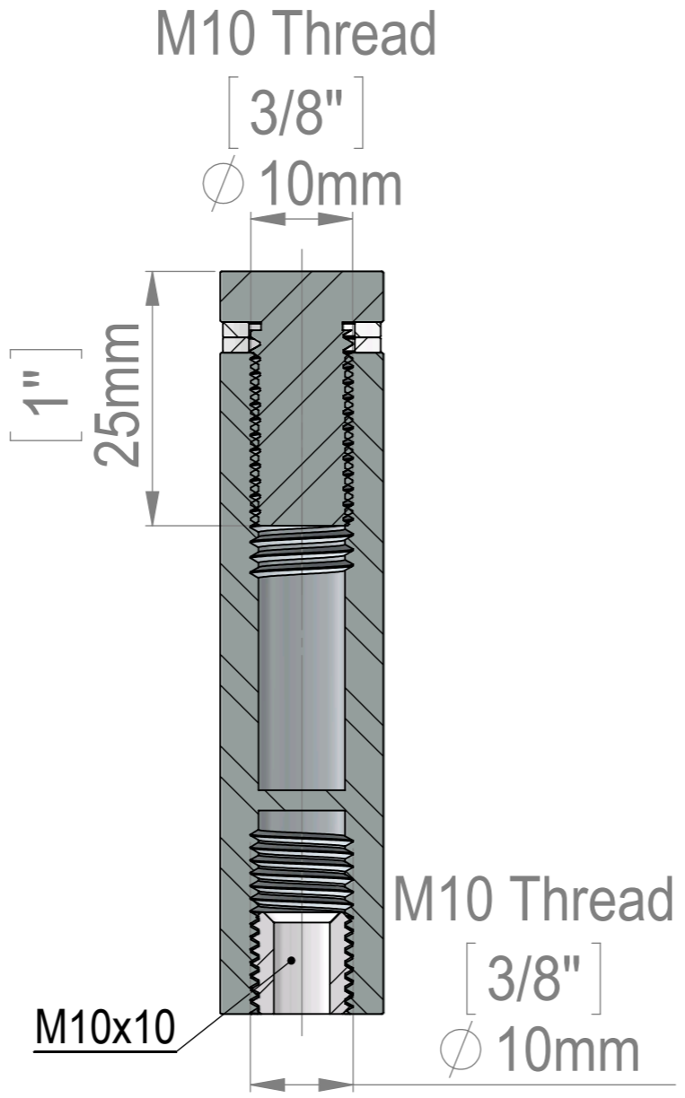
SECTION F-F SCALE 1.5 : 1
