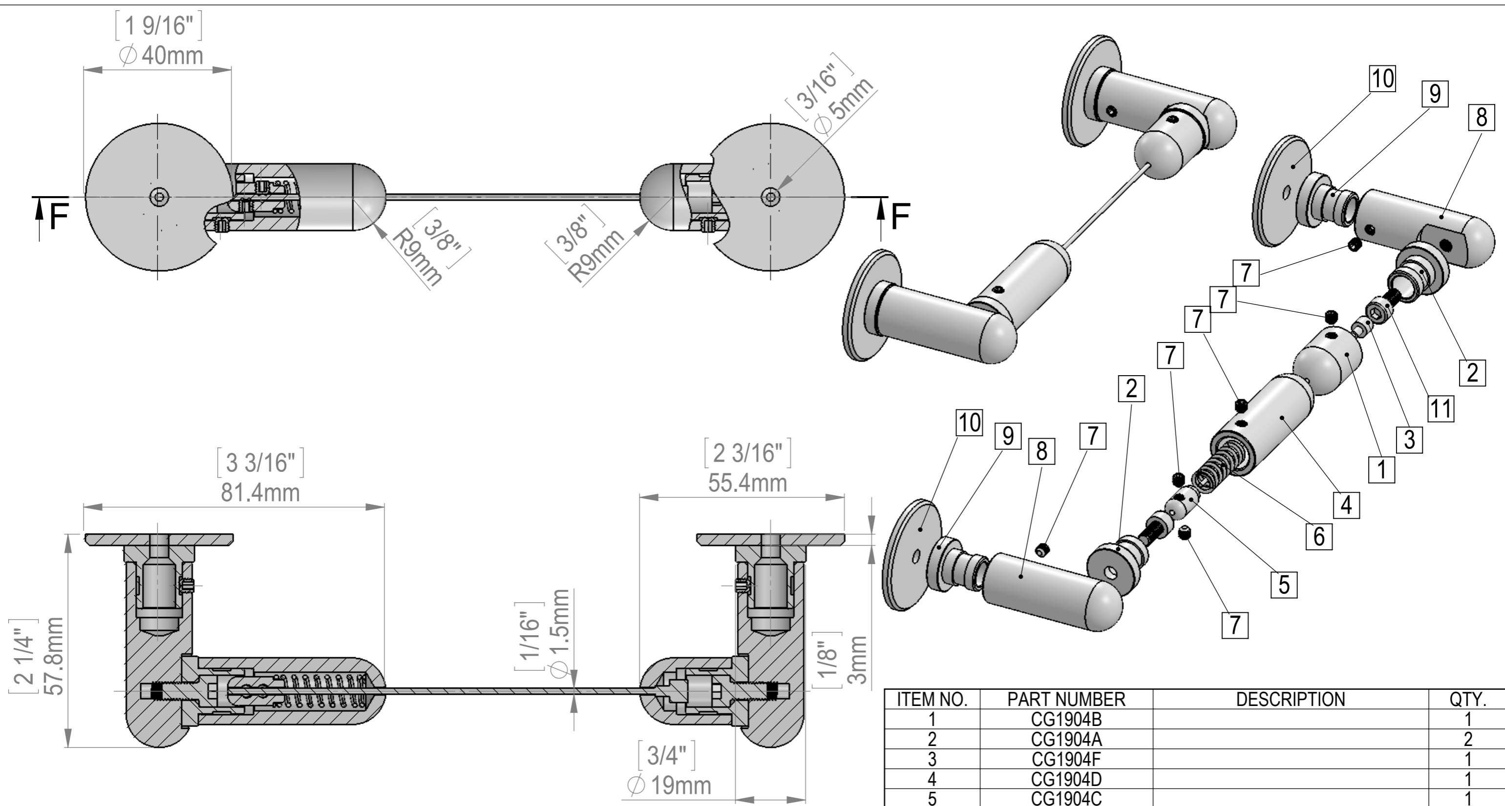
SECTION F-F SCALE 1 : 1
